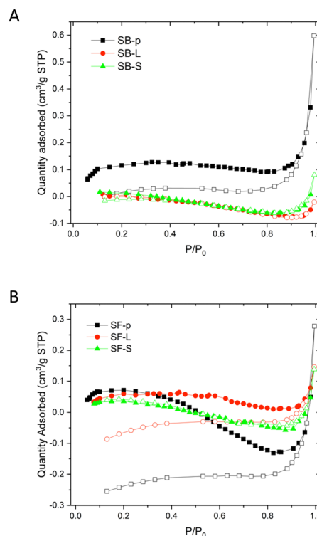
Fig. 6 Isotherms obtained from sphere derived samples showing negligible or no gas adsorption. (A) Granules derived from 3D printed sphere blocks: large (SB-L); small (SB-S); pulverized (SB-p). (B) Granules from sphere foam blocks: large (SF-L); small (SF-S); pulverized (SF-p).
