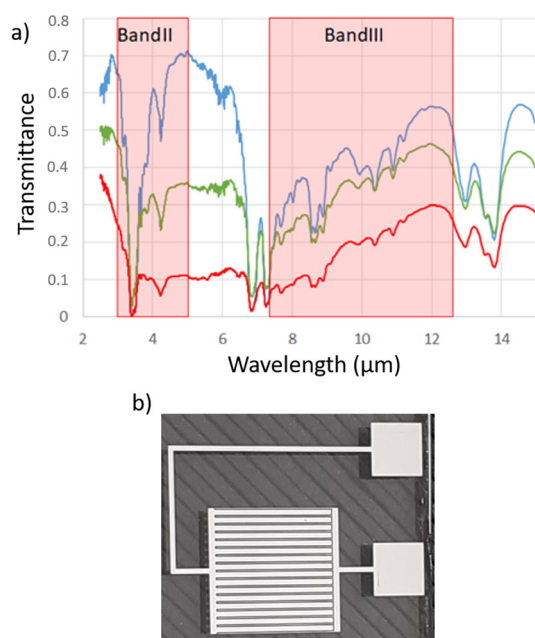
Fig. 5 (a) IR spectrum of Isopar L (blue), NP AZO at 10 \text{ mg mL}^{-1} (green) and 40 \text{ mg mL}^{-1} in Isopar L. (b) Optimized interdigit electrodes with 63% reflective surface and 50 \text{ }\mu\text{m} gap between electrodes.
