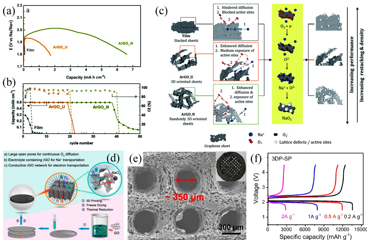
Fig. 5 (a) Discharge curves of three different electrodes at the current density of 100 \text{ mA g}^{-1} . (b) The evolution of discharge capacity and Coulombic efficiency with the number of cycles for the three different electrodes. (c) Schematic illustration of the proposed mechanism for the three different electrodes. (Reproduced from ref. 77 with permission from the Royal Society of Chemistry). (d) Schematic illustration of the 3D-rGO air electrodes for Na–O 2 battery. (e) SEM image of the 3DP-SP sample. (f) The initial discharge/charge curves of 3DP-SP cathodes at current density. (Reproduced from ref. 14 with permission from the American Chemical Society).
