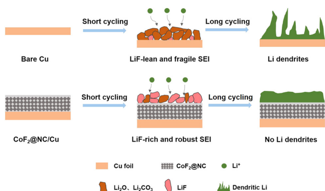
Fig. 7 Schematic illustration of the Li stripping/plating cycling on (a) bare Cu and (b) \text{CoF}_2\text{@NC/Cu} current collectors.
