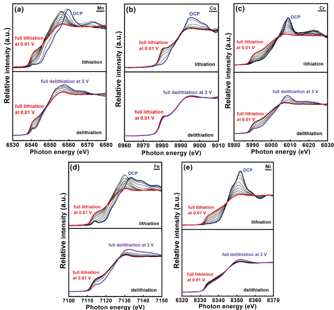
Fig. 7 Operando XAS spectra of HEO anode obtained during first lithiation/delithiation process at 150 mA g -1 current density. The interval between spectra is 100 mA h g -1 . Copyright permission from Wiley, used from ref. 49.
