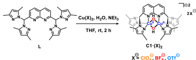
Scheme 1 Synthesis of C1(X) 2 complexes prepared in this work.
