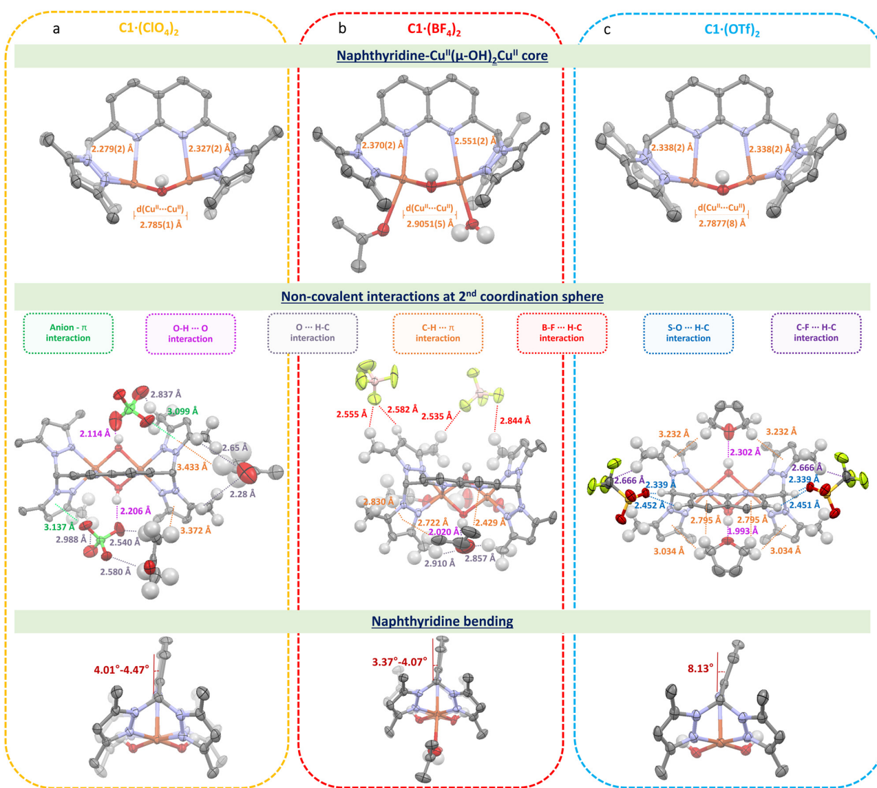
Fig. 1 Displacement ellipsoid plots of (a) C1 ·( \text{ClO}_4 ) 2 , (b) C1 ·( \text{BF}_4 ) 2 and (c) C1 ·( \text{OTf} ) 2 complexes at the 50% probability level. \text{Cu}-\text{N}_{\text{naph}} and \text{Cu} \cdots \text{Cu} distances (top), non-covalent interactions (middle) and naphthyridine bending angles (bottom). Solvent molecules, free anions and hydrogen atoms (except for the O-H bridges or when discussed) are omitted for clarity.
