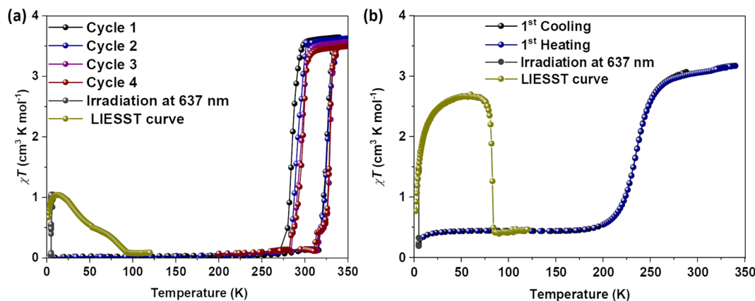
Fig. 6 Temperature- and light-induced spin-state switching of 1\text{-CH}_3\text{CN} and 2\text{b-CH}_3\text{CN-Y} . (a) \chi T versus T plots of wine-red crystals of 1\text{-CH}_3\text{CN} measured at a scan rate of 3 \text{ K min}^{-1} , showing temperature-dependent spin-state switching. Upon irradiation with 637 nm light at 5 K, the complex underwent light-induced LS-to-HS switching (grey filled circles) due to the LIESST effect. The green filled circles represent the temperature-dependent switching of the metastable HS state to the LS state. (b) \chi T versus T plot of complex 2\text{b-CH}_3\text{CN-Y} —the complex shows a gradual temperature-induced spin-state switching ( T_{1/2} = 234 \text{ K} ) with no thermal hysteresis. The complex also undergoes light-induced LS-to-HS switching (black filled circles), when irradiated with 637 nm light at 5 K. Temperature-induced conversion of the metastable HS state to the LS state starts around 50 K (green solid circles). A point noteworthy here is not only the thermal switching but also LIESST-mediated SCO is influenced by the nature of substituent, elucidating a connection between structural and spin isomerism.
