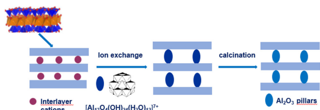
Fig. 1 Preparation of \text{Al}_2\text{O}_3 pillared clays.
