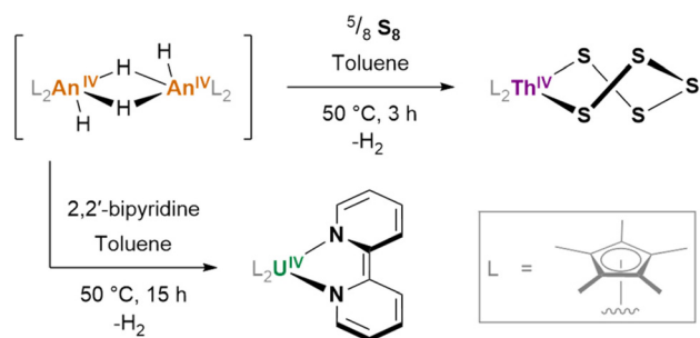
Fig. 21 Actinide hydride reduction behaviour towards substrates. (\text{Cp}^*\text{Th})_2(\text{H})_4 generated in situ reacts with elemental sulfur to yield form a \mu^5\text{-S}_8 coordinated product. The analogous uranium hydride, (\text{Cp}^*\text{U})_2(\text{H})_4 , reacts with 2,2'-bipyridine to coordinate the reduced bipyridyl dianion ( \text{bipy}^{2-} ).
