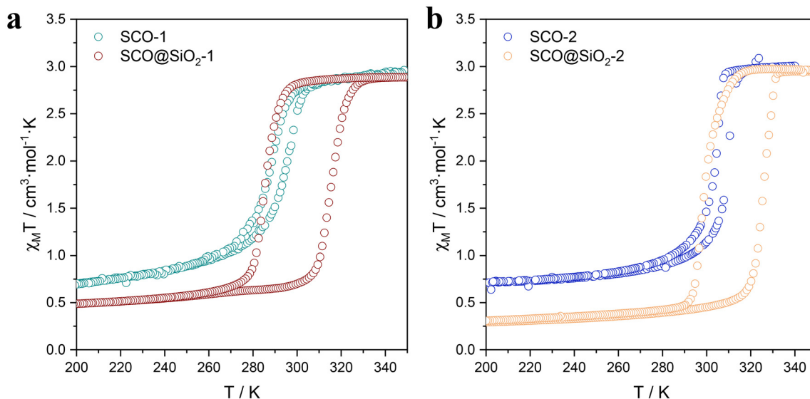
Fig. 3 Comparison of the thermal variation of the \chi_M T product for SCO-1 and \text{SCO@SiO}_2 -1 (a), and SCO-2 and \text{SCO@SiO}_2 -2 (b).
