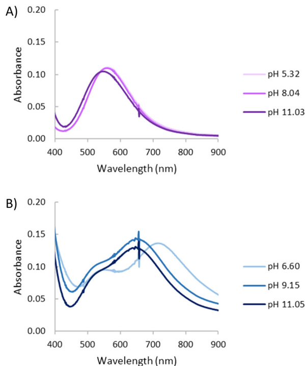
Fig. 8 UV-Vis spectra for the system \text{Cu}^{2+} – L1 at variable pH. (A) [\text{Cu}^{2+}] = [\text{L1}] = 1 \times 10^{-3} \text{ M} . (B) [\text{Cu}^{2+}] = 2 \times 10^{-3} \text{ M} , [\text{L1}] = 1 \times 10^{-3} \text{ M} .
