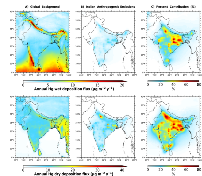
Fig. 8 Contributions of global background and Indian anthropogenic emissions to mercury wet (top panel) and dry deposition (bottom panel) during 2013–2017. (A) Absolute wet and dry deposition fluxes ( \mu\text{g m}^{-2} \text{ year}^{-1} ) due to global background emissions. (B) Absolute wet and dry deposition fluxes ( \mu\text{g m}^{-2} \text{ year}^{-1} ) due to Indian anthropogenic emissions. (C) Percentage contribution of Indian anthropogenic emissions to total wet and dry deposition.
