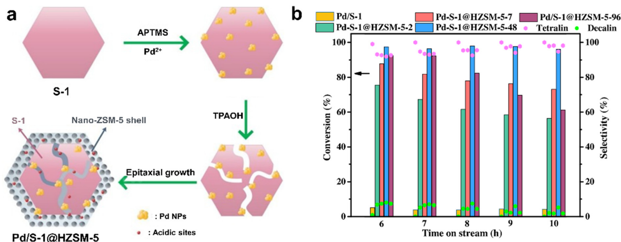
Fig. 14 (a) The preparation progress for the Pd/S-1@HZSM-5 catalyst; (b) catalytic performances of naphthalene hydrogenation over different catalysts (reaction conditions: WHSV = 1.3 h -1 , H 2 /feed = 750, 4 MPa H 2 , 280 °C). 118 Reprinted with permission from Elsevier B.V., copyright 2021.
