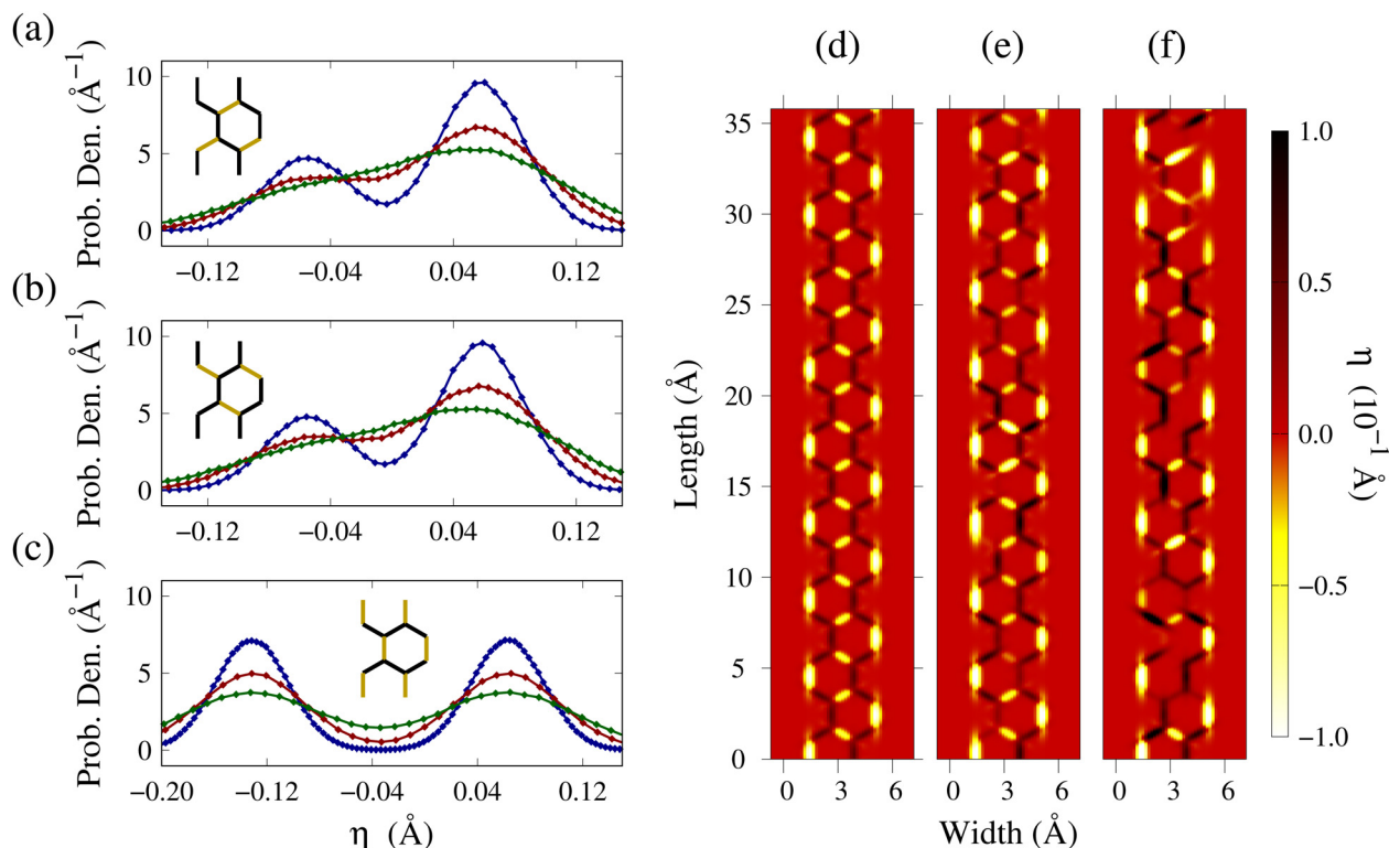
Fig. 2 Bond deformations in the presence of thermal effects in the neutral 4AGNR. (a), (b) and (c) are, respectively, the deformation distributions for the trans (/), cis (\) and vertical (|) bonds. In each plot, a GNR slice illustration is placed to exhibit, in yellow, the corresponding bond type. The blue, red, and green curves correspond to T = 95 , 197 , and 350 K. In addition, (d), (e), and (f) depict the bond deformation heatmaps for T = 0 , 95 , and 350 K. The dark colors refer to expanded bonds, while light tones indicate contraction.
