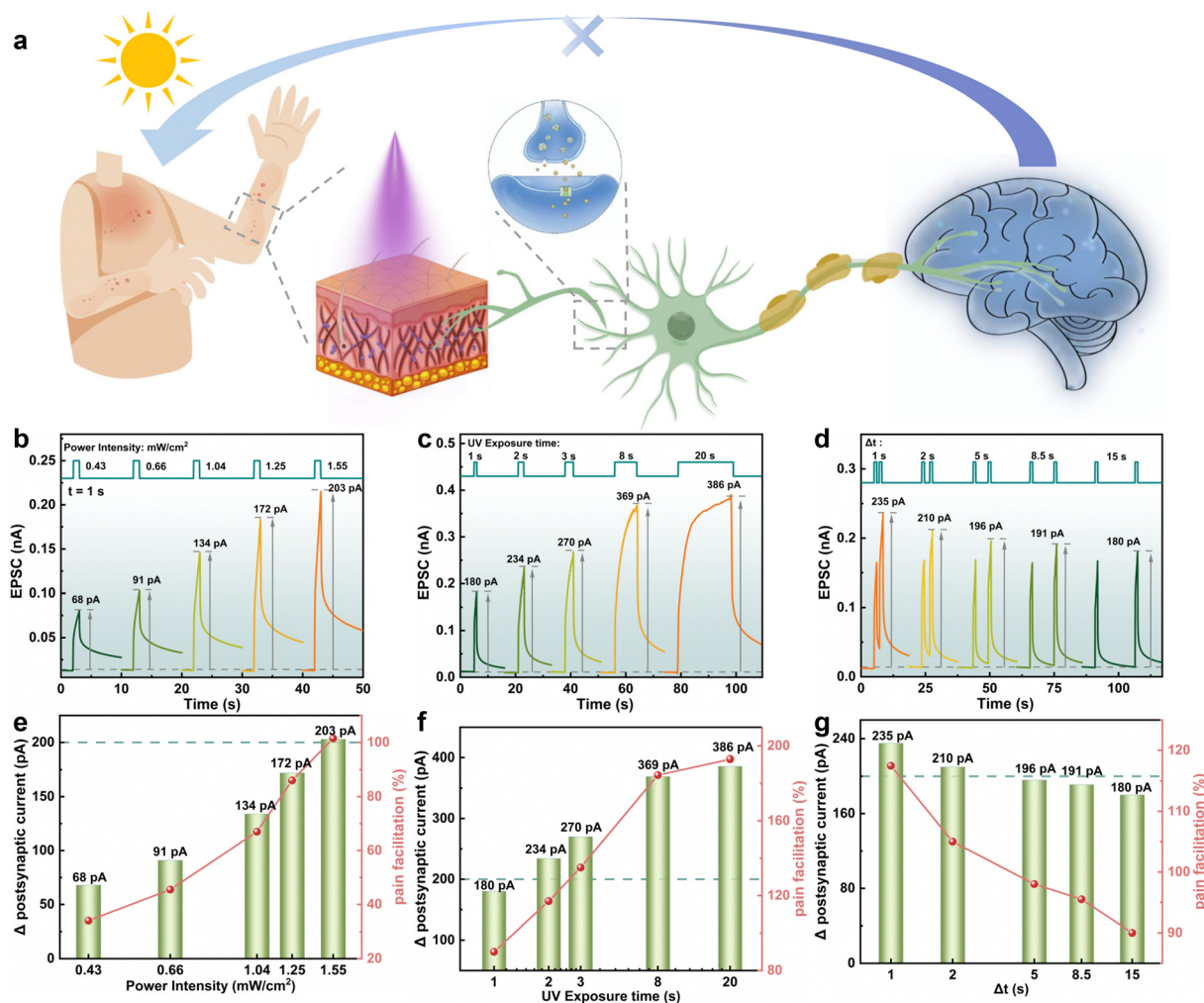
Fig. 4 (a) Schematic diagram of the device detecting, recognizing, and self-protecting against UV stimuli. (b) EPSC and (e) \Delta PSPC and pain facilitation under different UV irradiation intensities (320 nm, pulse width of 1 s). (c) EPSC and (f) \Delta PSPC and pain facilitation under different UV irradiation times (320 nm, 1.25 \text{mW cm}^{-2} ). (d) EPSC and (g) \Delta PSPC and pain facilitation under different UV irradiation intervals (320 nm, 1.25 \text{mW cm}^{-2} ).
