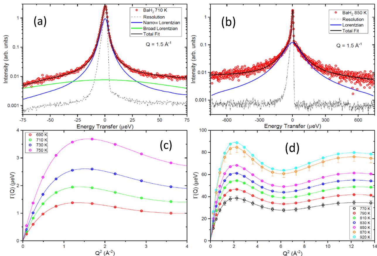
Fig. 8 The QENS measured for BaH 2 at BASIS (a) at T = 710 \text{ K} , and (b) at T = 850 \text{ K} . (c) and (d) show the HWHM at measured temperatures modeled with the Chudley-Elliott model. Reprinted with permission from 334 ( Sci. Rep. , 2022, 12 , 6194).
