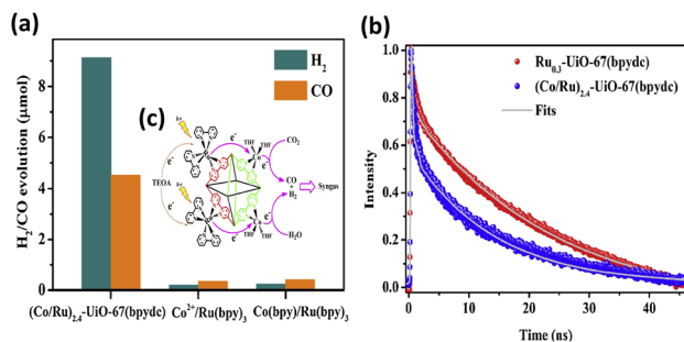
Fig. 2 (a) Results of photocatalytic \text{CO}_2 reduction under visible light illumination over (\text{Co/Ru})_{2.4}\text{-UiO-67(bpydc)} and the corresponding homogeneous counterparts. (b) Time-resolved PL spectra of (\text{Co/Ru})_{2.4}\text{-UiO-67(bpydc)} and \text{Ru}_{0.3}\text{-UiO-67(bpydc)} . Excitation and emission wavelength were 450 nm and 700 nm, respectively. (c) Proposed mechanism of interfacial charge transfer. Reproduced with permission from ref. 38. Copyright 2019, Elsevier.
