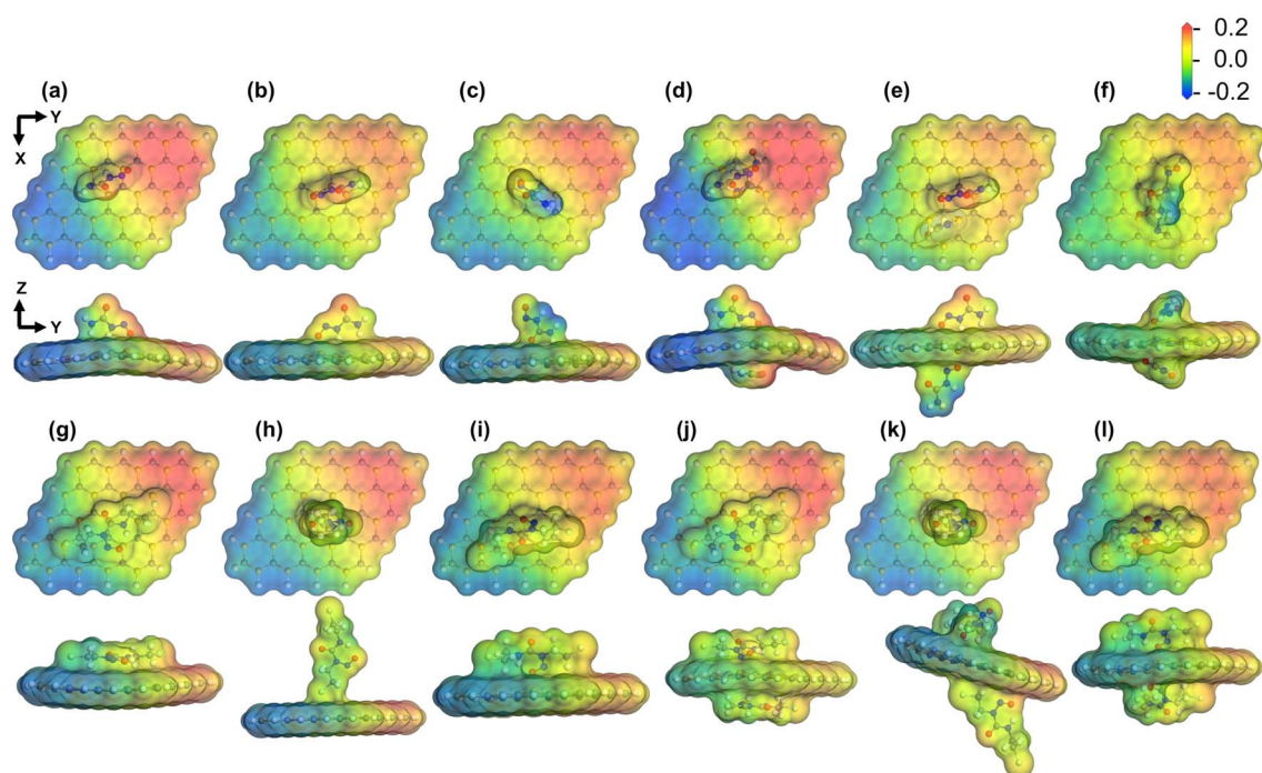
Fig. 8 COSMO surfaces (isovalue = 0.2 \text{ e} \text{ \AA}^{-3} ) for SiC/NU complexes (a) S1, (b) S2 (c) S3 (d) S4 (e) S5 and (f) S6 and SiC/BCNU complexes (g) S1, (h) S2 (i) S3 (j) S4 (k) S5 and (l) S6.
