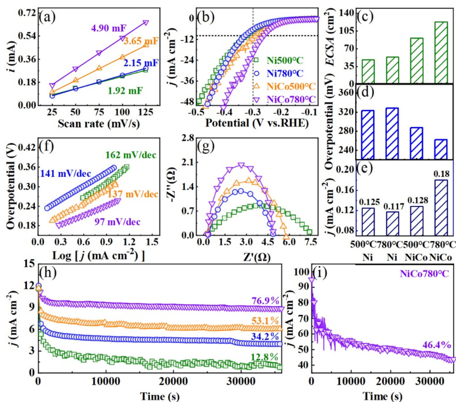
Fig. 6 (a) Electric double layer capacitance, (b) LSV curve, (c) ECSA, (d) overpotential at 10 \text{mA cm}^{-2} , (e) area activity at -0.3 V, (f) Tafel slope, and (g) electrochemical impedance of Ni and NiCo alloy catalysts. (h) Stability test of Ni and NiCo alloy catalysts at 10 \text{mA cm}^{-2} and (i) stability test of L 10 -NiCo alloys at 100 \text{mA cm}^{-2} .
