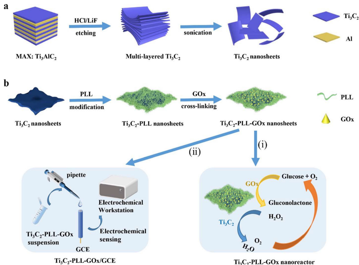
Fig. 9 The synthesis procedure and glucose detection mechanism of the \text{Ti}_3\text{C}_2 -PLL- \text{GO}_x bio-sensor, (a) synthesizing process and (b) detection mechanism. 168
