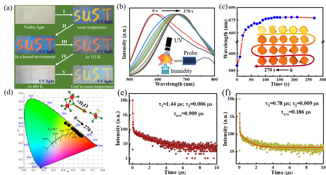
Fig. 3 Sensitivity of \text{Cs}_2\text{InBr}_5(\text{H}_2\text{O})\text{Sb}^{3+} to water molecules. (a) Digital photograph of “SUST” under various conditions. (b) PL spectra variation in a humid environment; the illustration depicts the in situ testing process of PL. (c) Peak position as a function of exposure time to a humid environment (inset showing the color change of the sample’s emission from 0 to 270 s). (d) CIE chromaticity diagram of the sample in a humid environment. The time-resolved PL decay curve for (e) \text{Cs}_2\text{InBr}_5(\text{H}_2\text{O})\text{Sb}^{3+} and (f) \text{Cs}_3\text{In}_2\text{Br}_9 .
