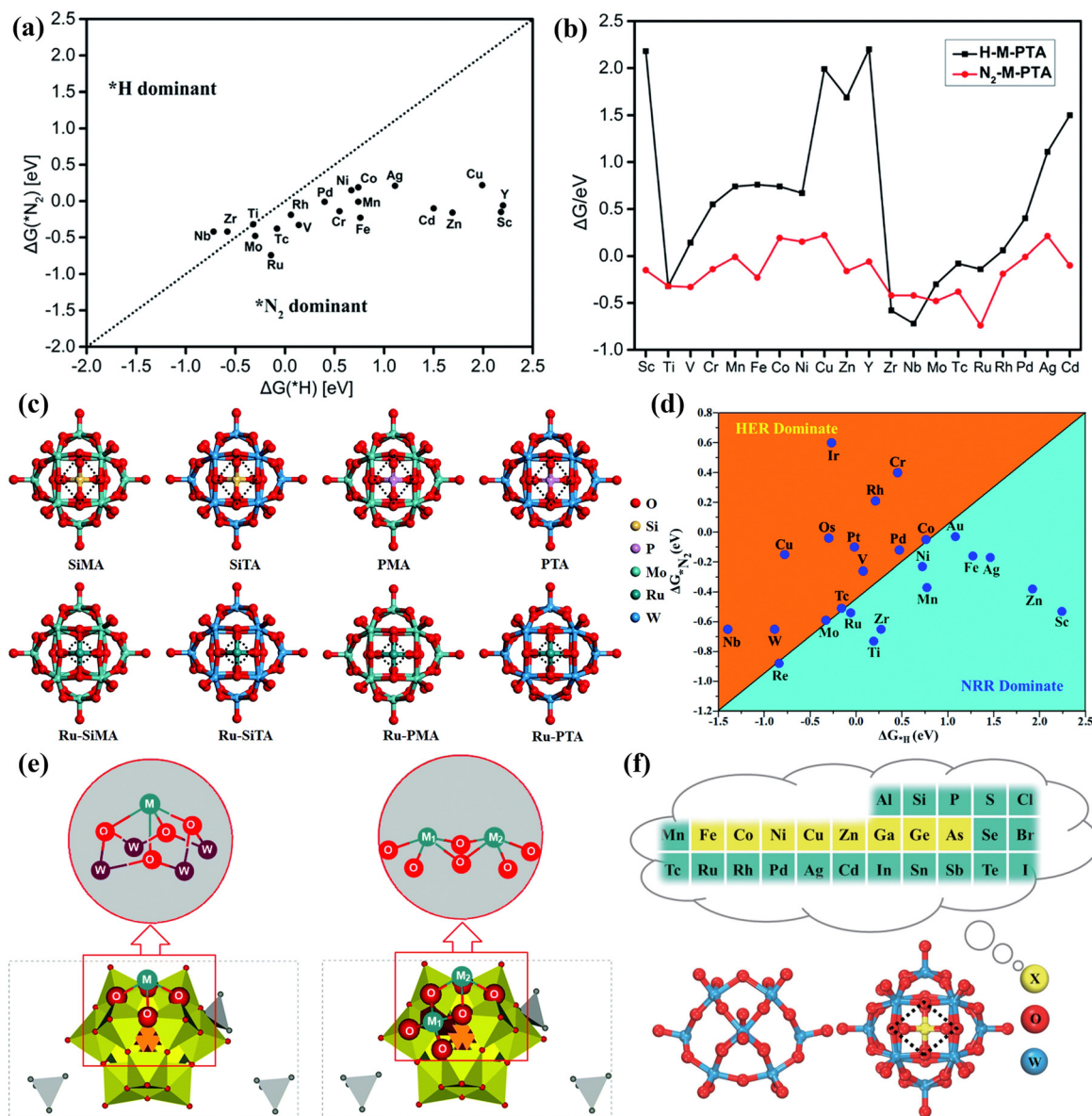
Fig. 17 (a) The calculated \Delta G^*(\text{N}_2) and \Delta G^*(\text{H}) on M-PTA. (b) The Gibbs free energy of *N 2 and *H adsorbed on M-PTA. 171 Copyright 2019, Royal Society of Chemistry (RSC). (c) Optimized structures of POM and Ru-POM. 172 Copyright 2020, Royal Society of Chemistry (RSC). (d) Calculated Gibbs free energies of N 2 and H 2 adsorbed on the M 1 /PMA cluster. 173 Copyright 2022, Royal Society of Chemistry (RSC). (e) The structure of [N(CH 3 ) 4 ] + [Ta II 2 /POM] (POM = [PW 11 O 39 ] 7- ). 174 Copyright 2022, Royal Society of Chemistry (RSC). (f) Optimized structures of POM. 175 Copyright 2023, Springer, Tsinghua University Press 2022.
