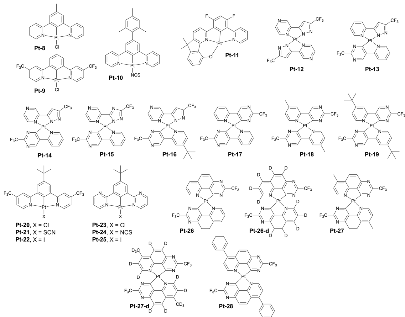
Fig. 9 Examples of aggregating platinum(II) complexes with long wavelength NIR photo- and electrochromic in neat films.
