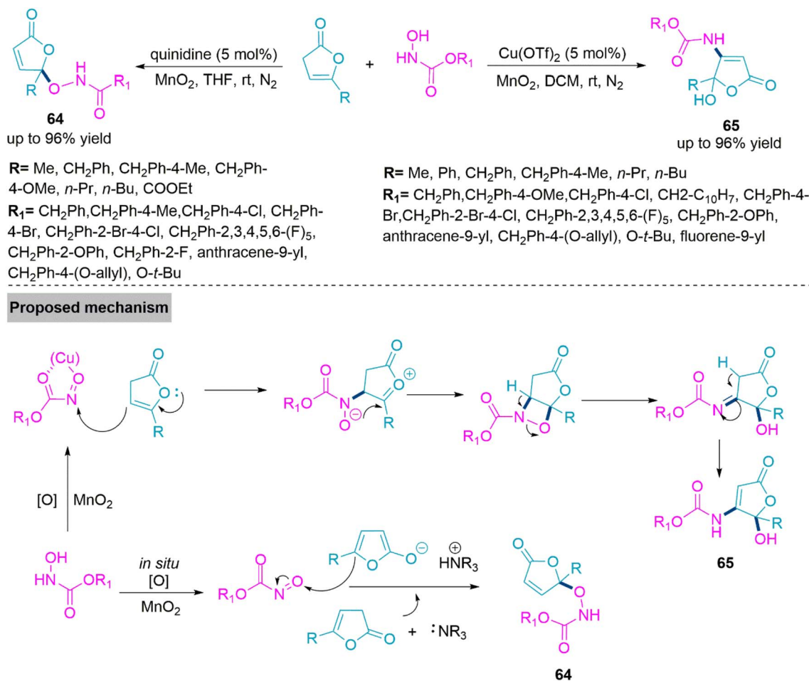
Scheme 34 Synthesis of γ-aminoxylation derivatives ( 64 ) and β, γ-disubstituted butanolide derivatives ( 65 ).
