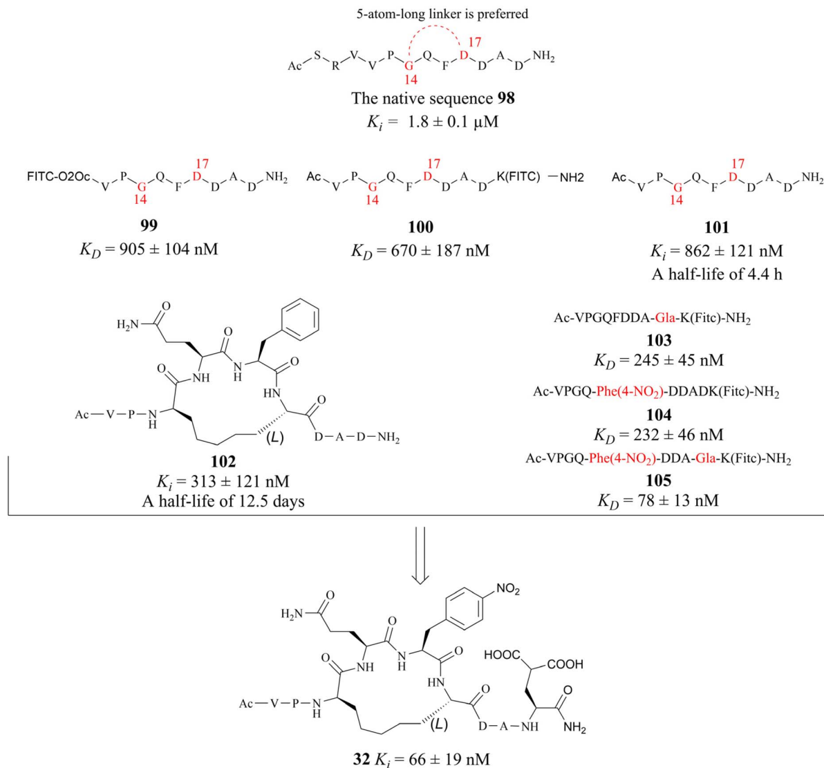
Fig. 15 Macrocyclization of the RioK1-derived PBM sequence results in a PAP11 32 .
