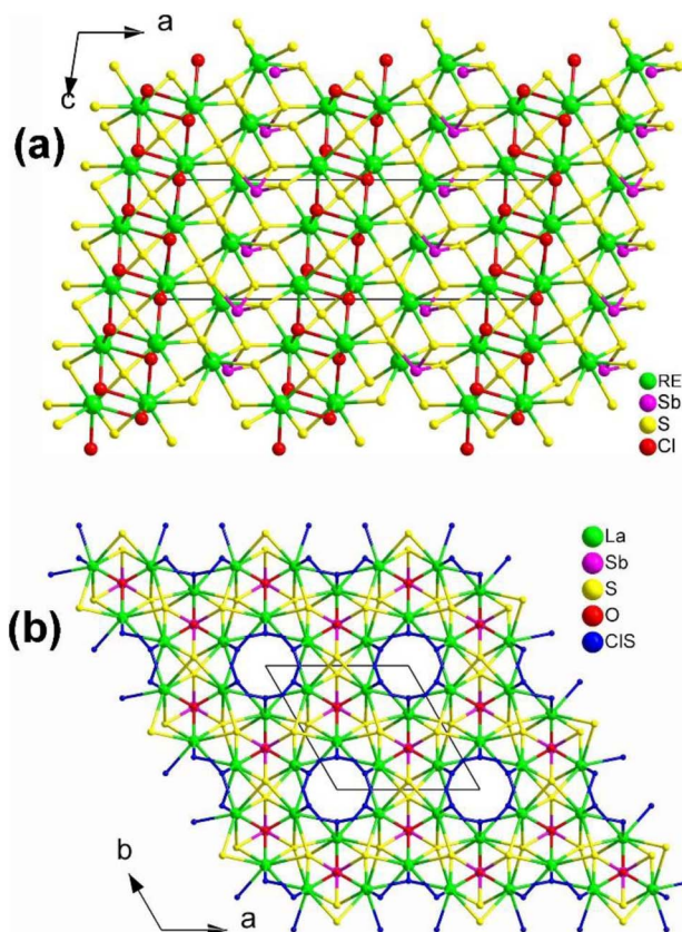
Fig. 24 Structures of (a) [\text{RE}_3\text{S}_2\text{Cl}_2][\text{SbS}_3] along the ac plane and (b) [\text{La}_3\text{OSCl}_2][\text{SbS}_3] along the ab plane with unit cell outlined.
