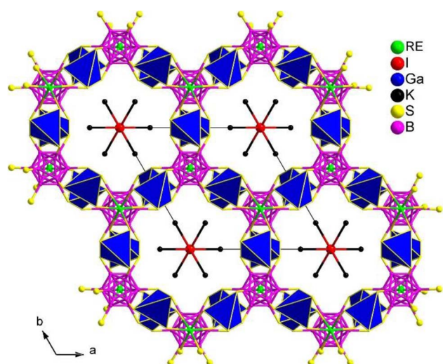
Fig. 23 Structure of (\text{K}_3\text{I})[\text{REB}_{12}(\text{GaS}_4)_3] with the unit cell outlined along the ab plane.
