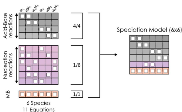
Fig. 1 Schematic example of the equations arising from a simple reaction network for one monomer M_1 giving a dimer M_2 , and their protonated forms, so a total of 6 species, 4 acid/base reactions in grey, 6 nucleation reactions in purple, plus the mass balance equation in orange.
