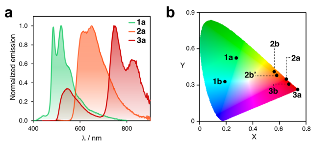
Fig. 5 (a) Emission spectra of complexes 1a, 2a, and 3a in DCM at 25 °C. (b) CIE plot of selected Pt II and Pt IV cyclometalated complexes containing ligands 1, 2 and 3. Data corresponding to DCM solutions recorded at 25 °C.
