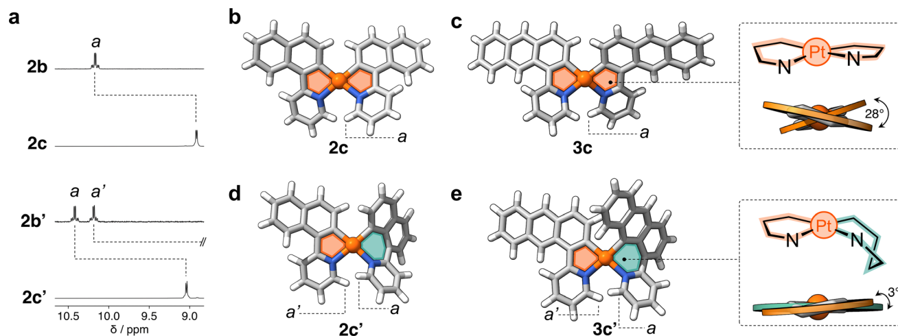
Fig. 4 (a) Partial 1 H NMR spectra (400 MHz, DCM- d 2 ) of complexes 2c and 2c' and their precursors 2b and 2b'. (b) Crystal structures as determined by SCXRD of complexes (b) 2c, (c) 3c, and DFT-minimized structures of (d) 2c' and (e) 3c'. Panels (c) and (e) depict the conformation of the 5- and 6-membered metallacycles as well as the dihedral angles in complexes 3c and 3c'.
