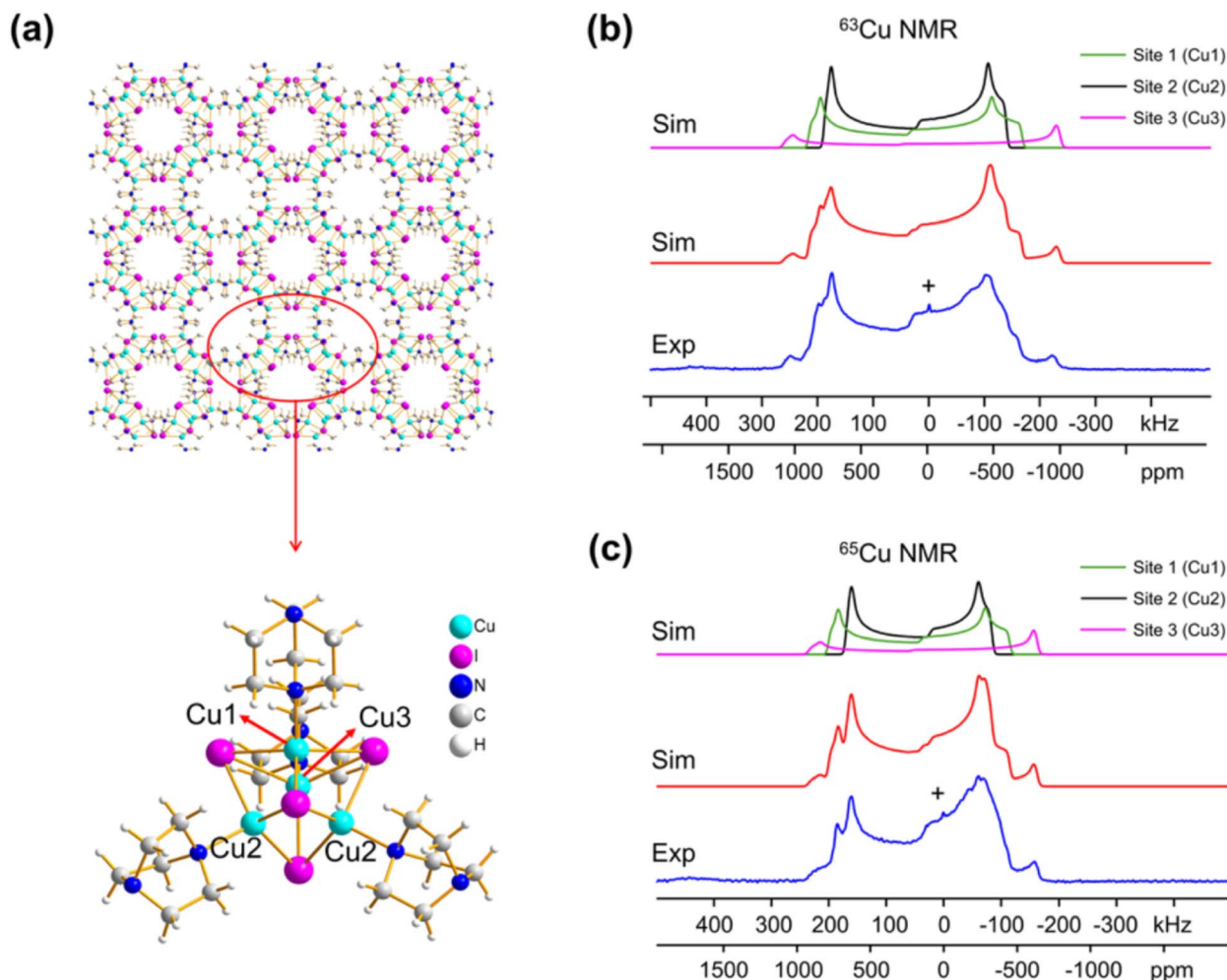
Fig. 1 (a) A schematic diagram of [Cu 4 I 4 (DABCO) 2 ] featuring three different Cu sites. The experimental (b) 63 Cu and (c) 65 Cu static NMR spectra (blue), cumulative simulations (red), and individual Cu site simulations (black, purple, green).
