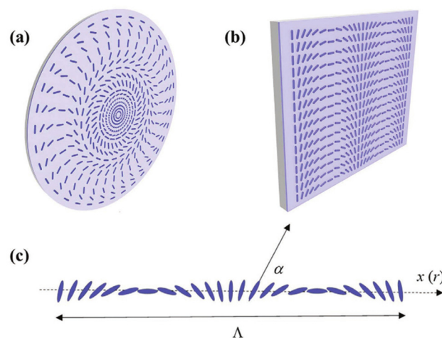
Fig. 1 Azodyne alignment patterns for 4G optical lens (a) and prism (b). The angle \alpha describing molecular orientation varies linearly along a Cartesian coordinate x for a prism (c) and it is a parabolic function of the radial coordinate r for a lens. Reproduced from ref. 1 with permission from John Wiley & Sons, copyright 2021.
