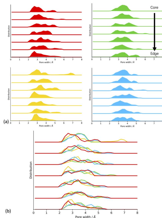
Fig. 7 (a) Plots of the pore size distributions calculated after network generation and desolvation for each solvent summed over each respective solvent model. (b) Comparison of the different solvent model pore size distributions. Stacked with increasing distance from the cluster edge to the core. Key: toluene – blue, THF – yellow, 1,4-dioxane – green, DMF – red.
