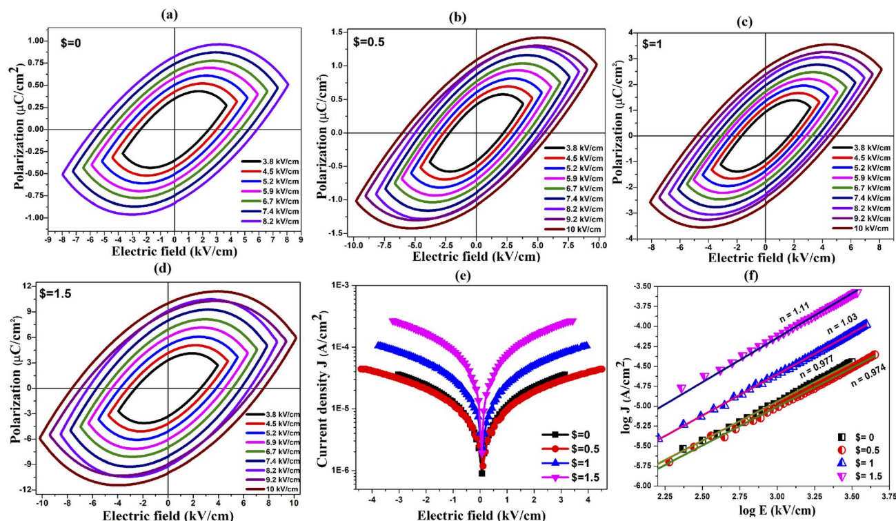
Fig. 5 (a)–(d) P – E curves for the 0.5BZT–0.5CNF– \% GO ( \% = 0, 0.5, 1, 1.5 ) composite at varying applied electric fields, (e) current density as a function of electric field for composites and (f) \log J vs. \log E graph for 0.5BZT–0.5CNF– \% GO ( \% = 0, 0.5, 1, 1.5 ).
