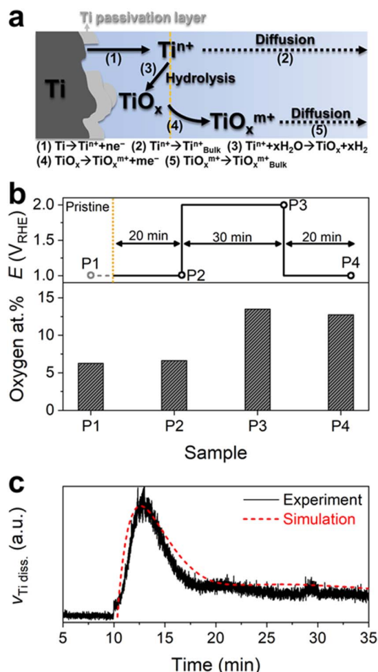
Fig. 3 (a) Schematic representation of the expected Ti PTL dissolution mechanism under highly anodic conditions. The reaction equation of each step is also shown. (b) Oxygen atomic percentages on the Ti PTL before (P1; gray circle) and after specific potential application (P2, P3, and P4; black circles) in \text{O}_2 -saturated 0.1 M \text{HClO}_4 . Oxygen content was estimated by EDS analysis. (c) Comparison of experimental and simulated Ti dissolution profiles at 2 V_{\text{RHE}} .
