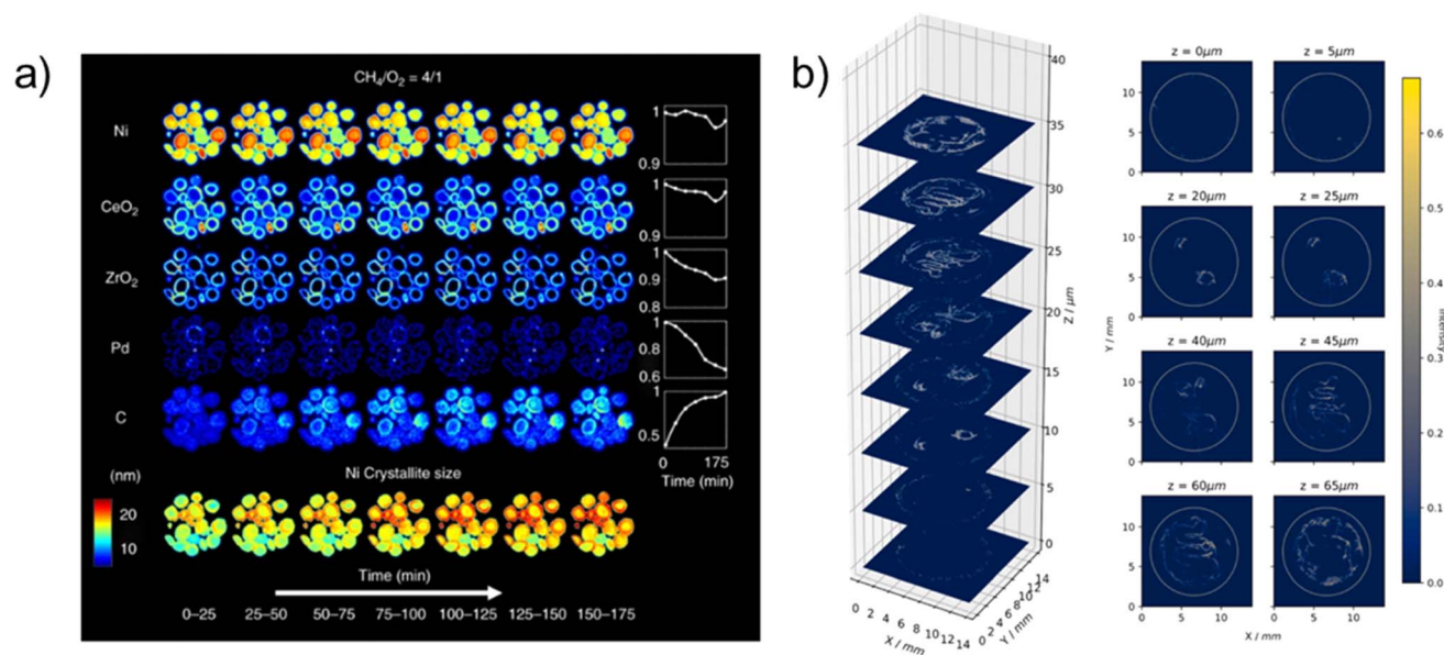
Fig. 7 (a) (Top): Synchrotron XRD-CT reconstruction showing chemical evolution of the complex \text{Ni-Pd/CeO}_2\text{-ZrO}_2/\text{Al}_2\text{O}_3 catalyst during partial oxidation of methane. Phase distribution maps of Ni, \text{CeO}_2 , \text{ZrO}_2 , Pd and C are derived from Rietveld analysis. (Bottom): Crystallite size map of Ni, displaying the change in crystallite size, collected during partial oxidation of methane experiment. Reprinted under the terms of the Creative Commons Attribution 4.0 International (CC-BY 4.0) license, from Vamvakeros et al. , 118 Copyright 2018, The Author(s), published by Springer Nature. (b) XRD-CT scan of the MEA's Cu catalyst layer, demonstrating the versatile high energy X-ray transparent \text{CO}_2 electrolysis cell for operando WAXS/SAXS-CT measurements. The plotted intensity correspond to the surface oxide ( \text{Cu}_2\text{O} ) XRD with one voxel resolution of 69.5 \mu\text{m} and the slice dimensions of 200 \times 200 voxels ( 13.9 \times 13.9 \text{ mm}^2 ). Reprinted from Moss et al. , 86 Copyright 2023, with permission from Elsevier.
