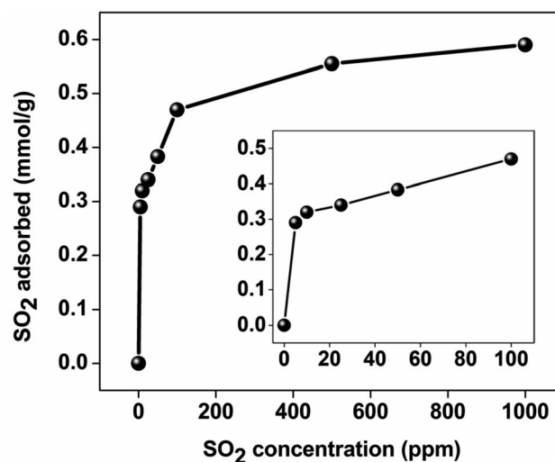
Fig. 5 \text{SO}_2 adsorption isotherms of GD-PEI/S.
