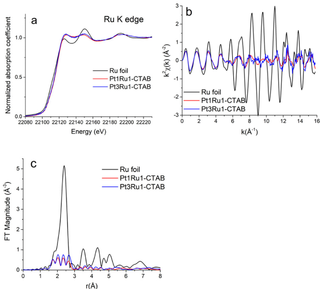
Fig. 5 (A) Ru K-edge XANES data. (B) k^2 -weighted EXAFS data in k -space. (C) Fourier transform magnitudes of the k^2 -weighted EXAFS data for Ru foil, Pt_1Ru_1 (produced with CTAB), and Pt_3Ru_1 (generated with CTAB).
