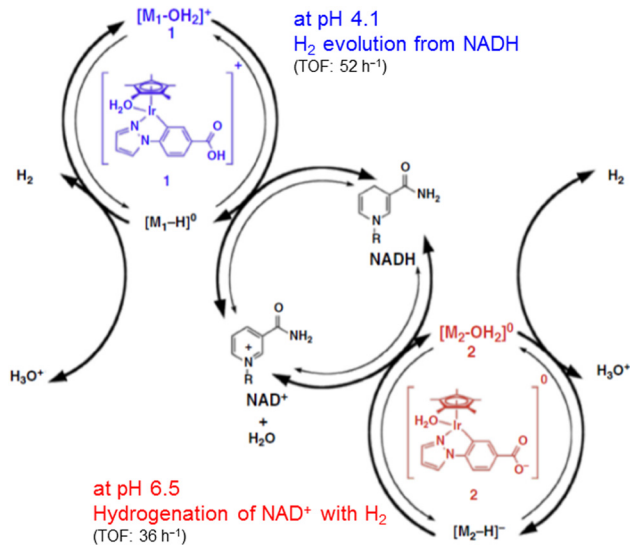
Scheme 10 Proposed mechanism for catalytic interconversion between NADH and H 2 with use of water soluble [C,N] cyclometalated Ir complexes ( 1 and 2 ) depending on pH. Reproduced with permission from ref. 75. Copyright 2011, American Chemical Society.
