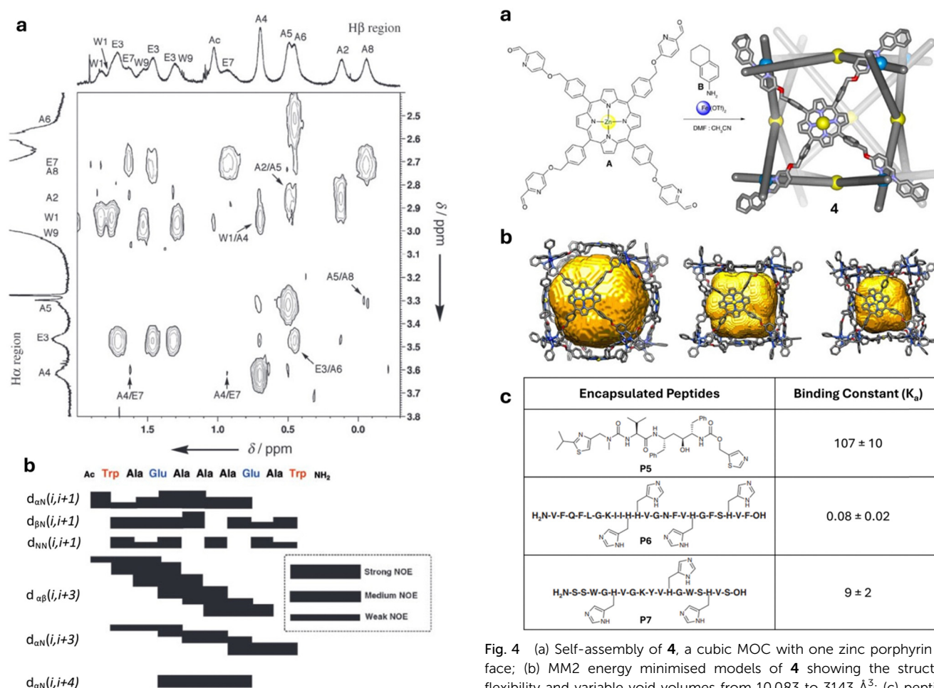
Fig. 3 (a) Selected NOESY spectrum for the assignment of bound peptide (600 MHz, H 2 O/D 2 O = 9/1, 27 °C, 100 mM phosphate buffer, pH 6.8), [2] = 10 mM, [peptide] = 2.5 mM. Proton resonances labelled with single letter amino acid code and residue number corresponding to peptide in Fig. 2a; (b) NOE correlations for peptide 2 . Reproduced with permission from ref. 16.
