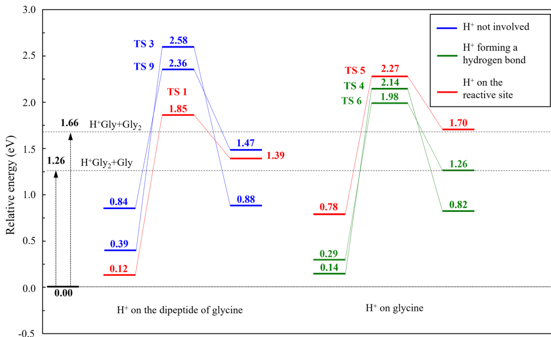
Fig. 6 Simplified reaction profiles summarizing the paths leading to protonated triglycine from the mixed dimer H^+Gly_2(Gly) in the cases where diglycine (left) or the glycine monomer (right) carries the excess proton. Only the energies of the initial, rate-determining transition and final states are shown.
