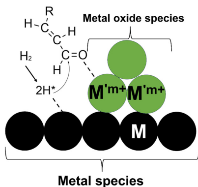
Scheme 2 Proposed reaction mechanism for unsaturated aldehyde hydrogenation and polyol hydrogenolysis over bimetallic \text{M}-\text{M}'\text{O}_x catalysts.
