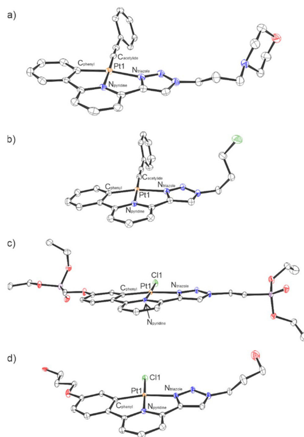
Fig. 2 Molecular structures of (a) [\text{Pt(A)}^M\text{L}] , (b) [\text{Pt(A)}^{\text{CL}}] (a co-crystallized \text{CH}_2\text{Cl}_2 molecule is omitted for clarity), (c) [\text{PtCl}^{\text{PL}^P}] , and (d) [\text{PtCl}^{\text{OHL}^{\text{OH}}}] (a co-crystallized DMF molecule (half a molecule in the asymmetric unit) is omitted for clarity) in the crystal. Displacement ellipsoids are drawn at the 50% probability level. H atoms are omitted for clarity.
