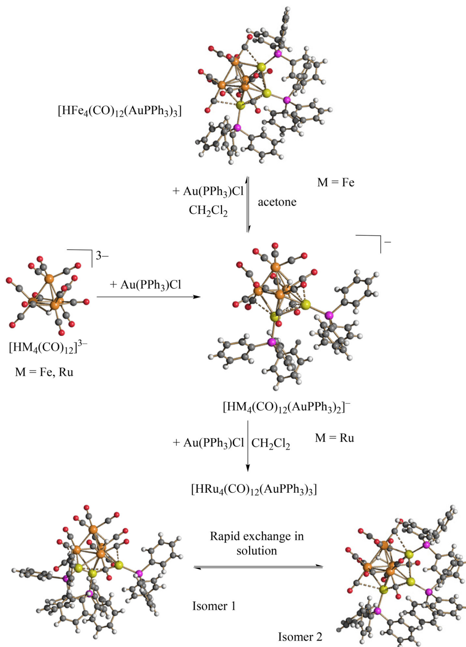
Fig. 2 Reactions of [\text{HM}_4(\text{CO})_{12}]^{3-} ( \text{M} = \text{Fe, Ru} ) with increasing amounts of \text{Au(PPh}_3\text{)Cl} result in the formation of [\text{HM}_4(\text{CO})_{12}(\text{AuPPh}_3)_2]^- and [\text{HFe}_4(\text{CO})_{12}(\text{AuPPh}_3)_3] . Anionic Fe and Ru clusters are isostructural, whereas noticeable differences are detected for the neutral clusters. [\text{HFe}_4(\text{CO})_{12}(\text{AuPPh}_3)_3] displays the unique hydride within the tetrahedral \text{Fe}_4 cavity, and its formation is reversed in polar solvents such as acetone. [\text{HRu}_4(\text{CO})_{12}(\text{AuPPh}_3)_3] exists as two isomers in rapid exchange in solution, both displaying the hydride ligand on the surface of the cluster (orange, Fe or Ru; yellow, Au; purple, P; red, O; grey, C; white, H).
