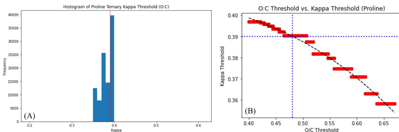
Fig. 1 O : C-LLPS threshold prediction results, where (A) \kappa_{\text{thresh}} frequency distribution after iterating 100 000 times and the most frequent bin ( \kappa_{\text{thresh}} ) shown by a red dashed line and (B) O : C thresh vs. \kappa_{\text{thresh}} , where the most frequent \kappa_{\text{thresh}} and its corresponding O : C thresh value are shown by the blue dotted lines. The corresponding O : C thresh value is the O : C threshold of the system, where the phase separation limit is most probable and thermodynamically favorable.
