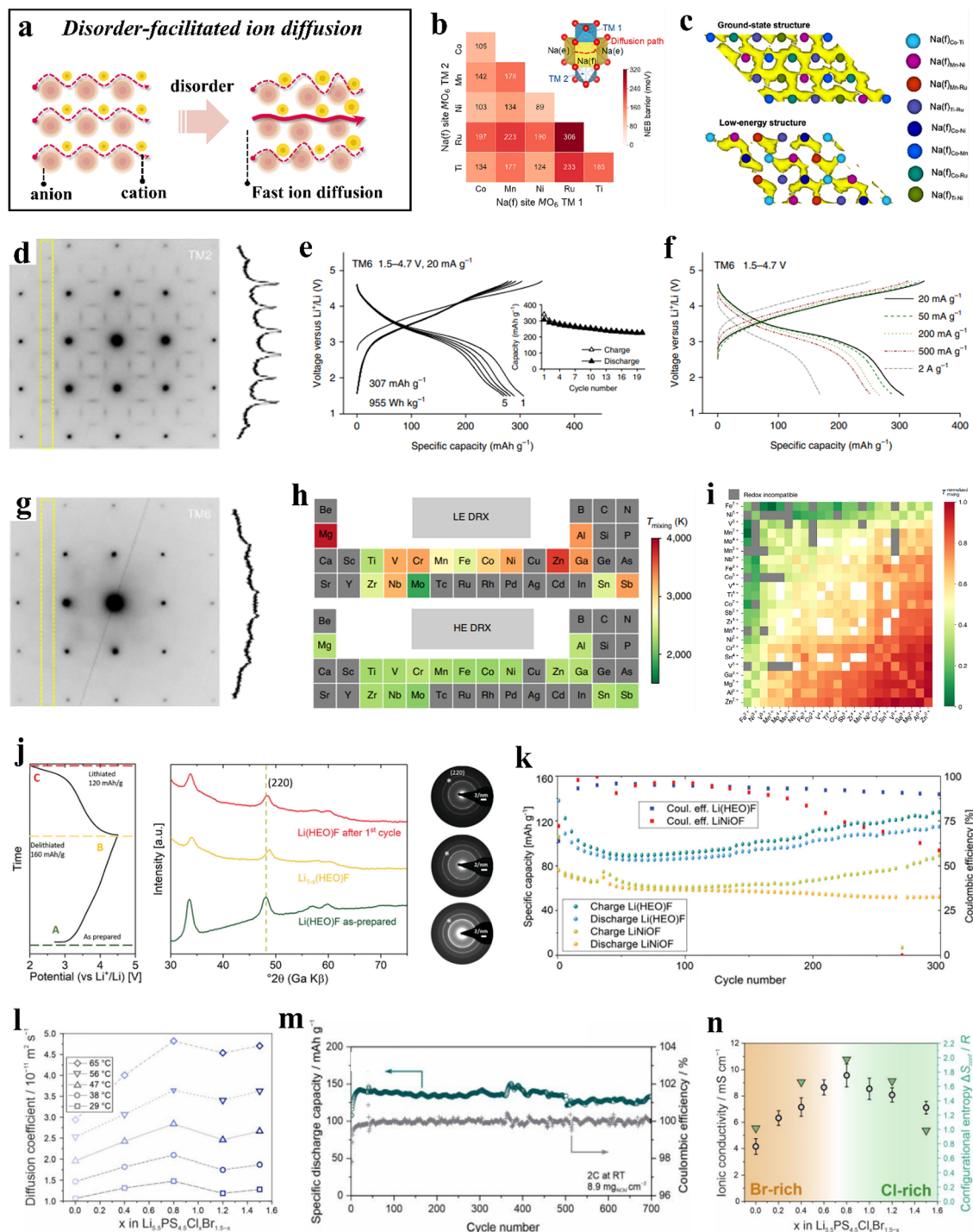
Fig. 7 (a) Schematic illustration of disorder-facilitated ion diffusion. (b) and (c) Theoretical calculations for P2-TMCNR. 273 (b) Na + migration barriers of different Na(f) M-TM . (c) AIMD trajectories for the ground-state structure and a low-energy structure. (d)–(i) DRX compounds. 211 (d) ED pattern collected from TM2 along the [100] zone axis. (e) Voltage profiles of TM6 within the potential window of 1.5–4.7 V at 20 mA g -1 . (f) Rate capability of TM6. (g) ED pattern collected from TM6 along the [100] zone axis. (h) Periodic table-type heat map of mixing temperatures of different elements in LE and HE DRXs. (i) Normalized mixing temperatures. (j) and (k) Li(HEO)F and LiNiOF cathodes. 276 (j) Initial charge/discharge curve at C/10 (20 mA g -1 ) in the potential range between 2.0 and 4.5 V (left) and the corresponding ex situ XRD patterns (middle), as well as ED data (right). (k) Comparison of capacity retentions at C/10 of Li(HEO)F and LiNiOF. (l)–(n) Li 5-x PS 4.5 Cl x Br 1.5-x electrolytes. 274 (l) Lithium-diffusion coefficients at different temperatures. (m) Capacity retention and Coulomb efficiencies. (n) Ionic conductivity as a function of x .
