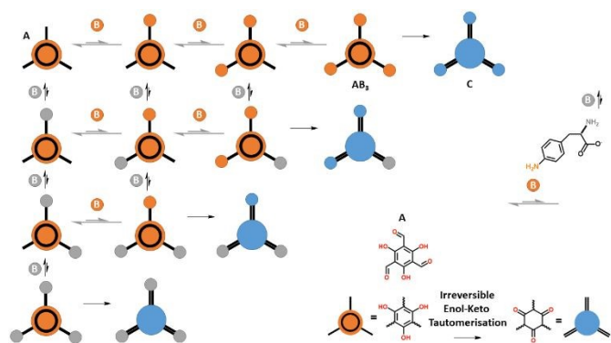
Figure 2. Reaction Network showing the thirteen possible products from the mixing of A (1,3,5-triformylglucinol) and B (4-amino- L -phenylalanine) in water at a pH of approximately 8. A can react with B through the aniline functional group (horizontal equilibrium arrows (orange)) or the alkyl amine functional group (vertical equilibrium arrows (grey)). Both equilibria are biased towards starting materials due to water. The irreversible enol-keto tautomerisation only occurs once all three aldehyde functional groups have reacted, shown as a horizontal reaction unidirectional arrow. Only the product C is analytically observed. It results from the tautomerisation of AB 3 (the thrice reacted aniline product).
