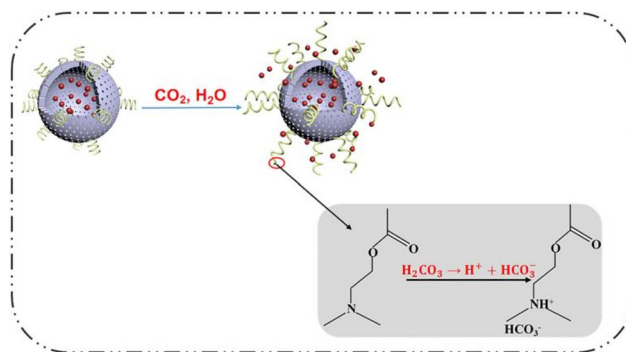
Fig. 17 Mechanism of the \text{CO}_2 stimulus response. Reproduced with permission 39 from Elsevier.
