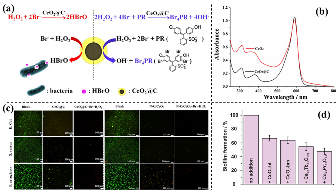
Fig. 4 (a) Reaction mechanism of \text{CeO}_2@\text{C} as a haloperoxidase mimic. 20 Reproduced from ref. 20 with permission from Elsevier, copyright 2020. (b) Absorbance spectra of solutions catalyzed by \text{CeO}_2@\text{C} and \text{CeO}_2 HS. 20 Reproduced from ref. 20 with permission from Elsevier, copyright 2020. (c) Live/dead staining images of E. coli , S. aureus and P. aeruginosa . 20,21 Reproduced from ref. 20,21 with permission from Elsevier and MDPI, copyright 2020 and 2023. (d) Crystal violet staining assay of P. aeruginosa grown in lysogeny broth. 22 Reproduced from ref. 22 with permission from RSC, copyright 2022.
