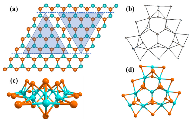
Fig. 1 (a) The equilibrium 2D monolayer MoTe 2 TMD with a Te–Mo–Te tri-layer structure. The two horizontal blue color dashed lines indicate terminations along the (1010) Mo-edge and (1010) Te-edge. The two triangles represent the terminations for Mo-edge and Te-edge clusters. It includes a non-periodic molecular cluster with an active Te-edge and a non-periodic molecular cluster with an active Mo-edge. (b) The molecular cluster model system of the 2D monolayer MoTe 2 TMD represented schematically. (c) A side view of the chosen Mo 10 Te 21 non-periodic triangular molecular cluster. (d) A top view of the MoTe 2 TMD Mo-edge cluster.
