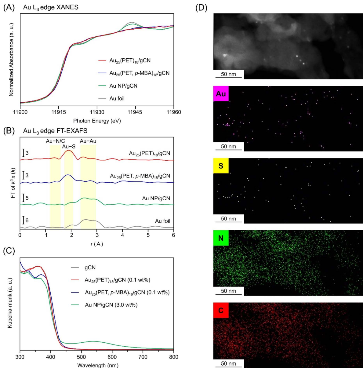
Fig. 3 Characterization of cocatalyst-loaded gCN photocatalysts. Au L_3 -edge (A) XANES, (B) FT-EXAFS spectra and (C) DR spectra. (D) HAADF-STEM images and EDS elemental mapping of \text{Au}_{25}(\text{PET})_{18}/\text{gCN} (Au-M, S-K, C-K and N-K). In (A and B), Au L_3 -edge XANES and FT-EXAFS spectra of Au foil is also shown for comparison. In (B), the peaks at \approx 1.9 and 2.6-3.0 Å are assigned to the Au-S and Au-Au bonds, respectively. Loading amounts of Au are 0.1, 0.1 and 3.0 wt% for \text{Au}_{25}(\text{PET})_{18}/\text{gCN} , \text{Au}_{25}(\text{PET}, p\text{-MBA})_{18}/\text{gCN} and Au NP/gCN, respectively.
