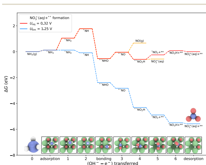
Fig. 16 Free energy diagram of \text{NO} (g), \text{NO}_2^- (aq), and \text{NO}_3^- (aq) formation by proceeding through the interaction between ^*\text{N} -containing intermediates and the lattice oxygen, ^{**}\text{O}_{\text{lat}} . It was calculated that the energies of desorption for \text{NO} (g), \text{NO}_2^- (aq), and \text{NO}_3^- (aq) is +0.77 , +0.19 , and -0.74 eV, respectively. Equilibrium (red trace) and limiting (blue trace) potentials are calculated using the computational hydrogen electrode at pH 11.
